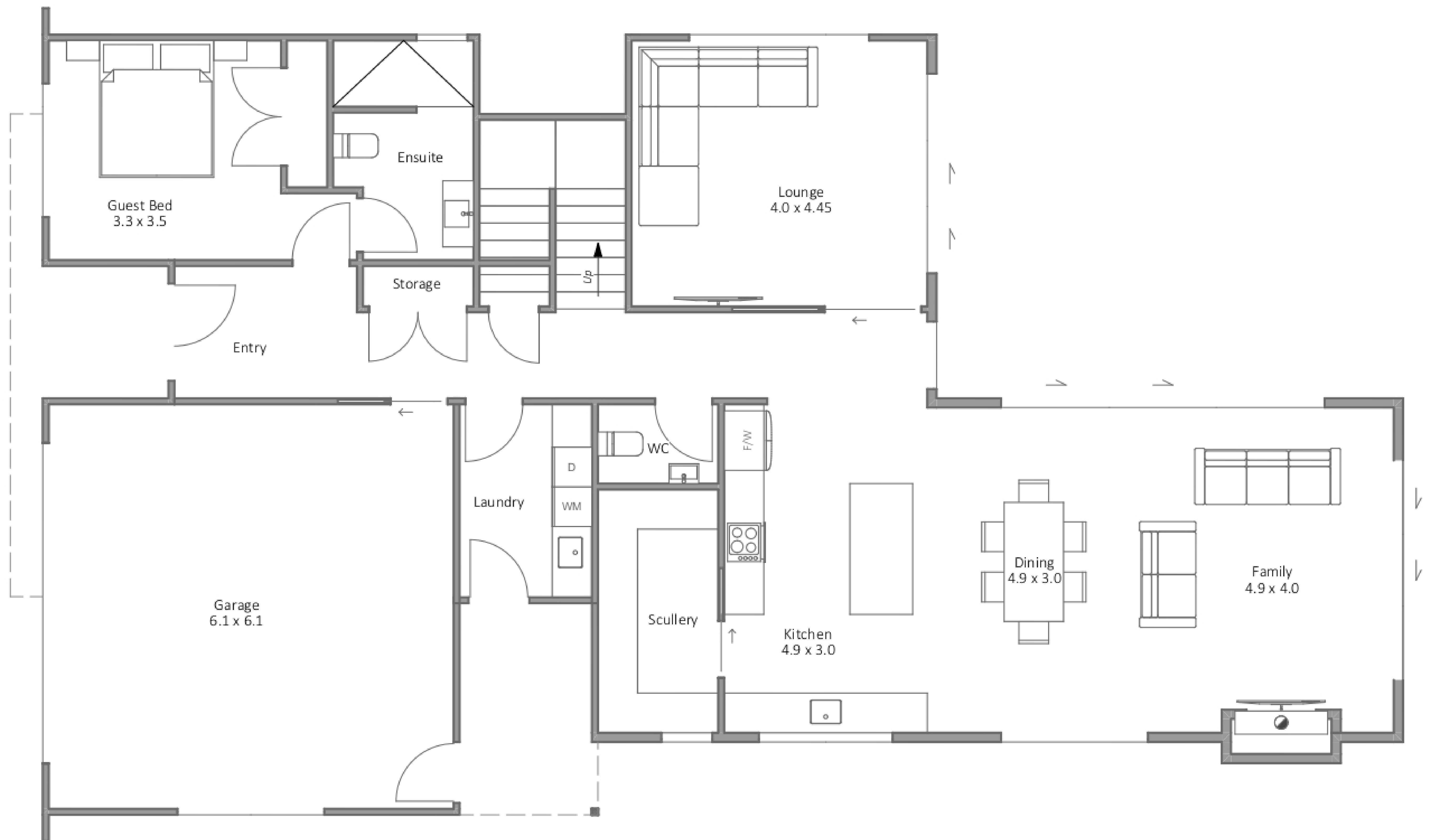
Ground Floor
