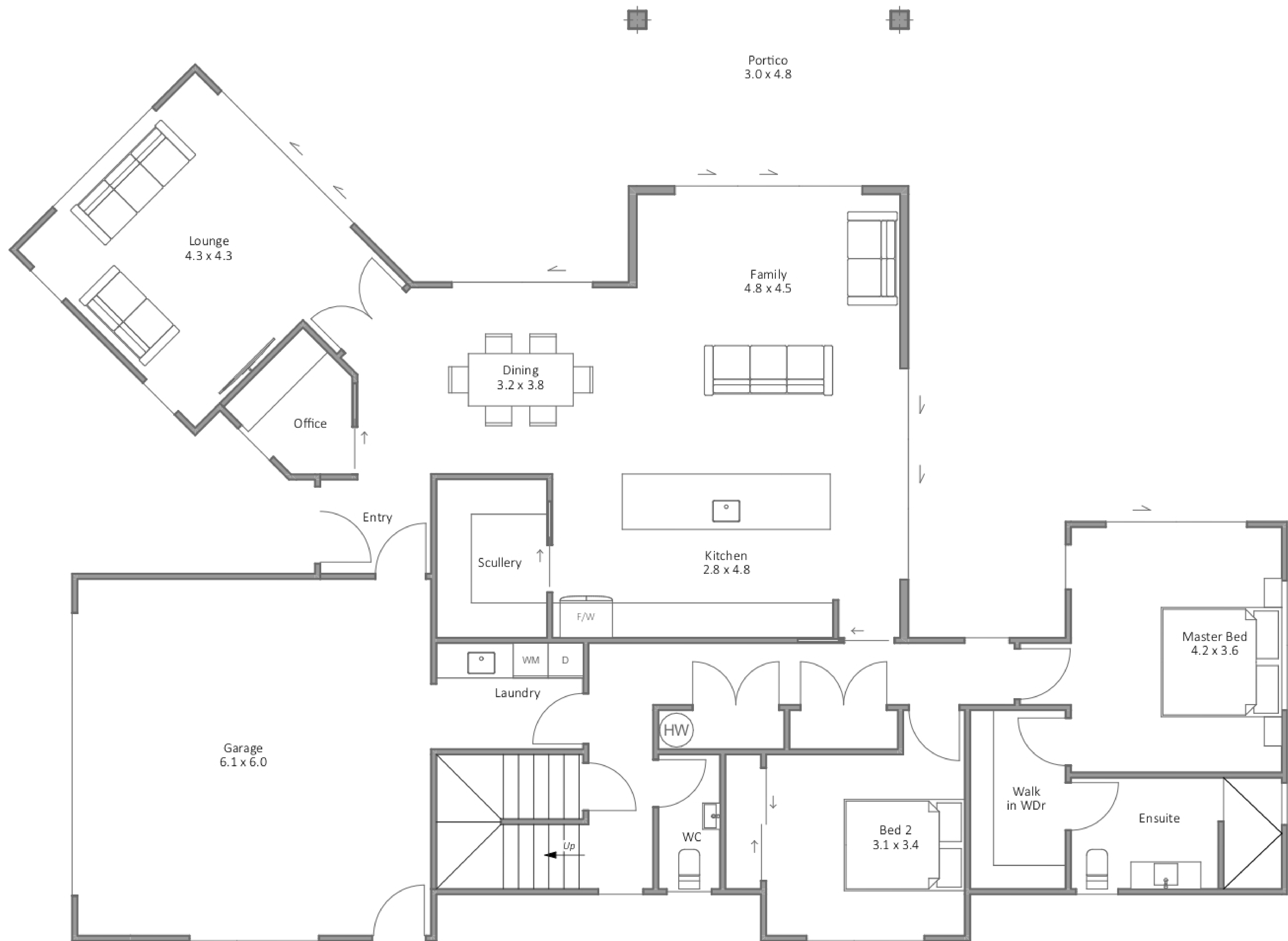
Ground Floor
